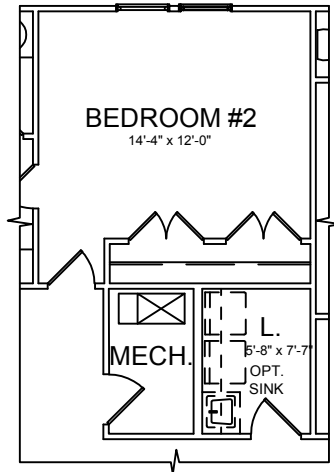
OPTIONAL SECOND FLOOR LAUNDRY
