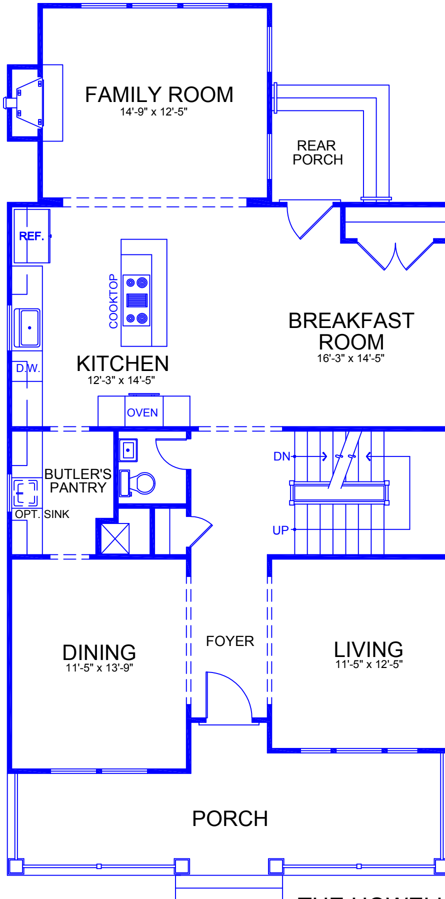
THE HOWELL MODEL FIRST FLOOR PLAN
